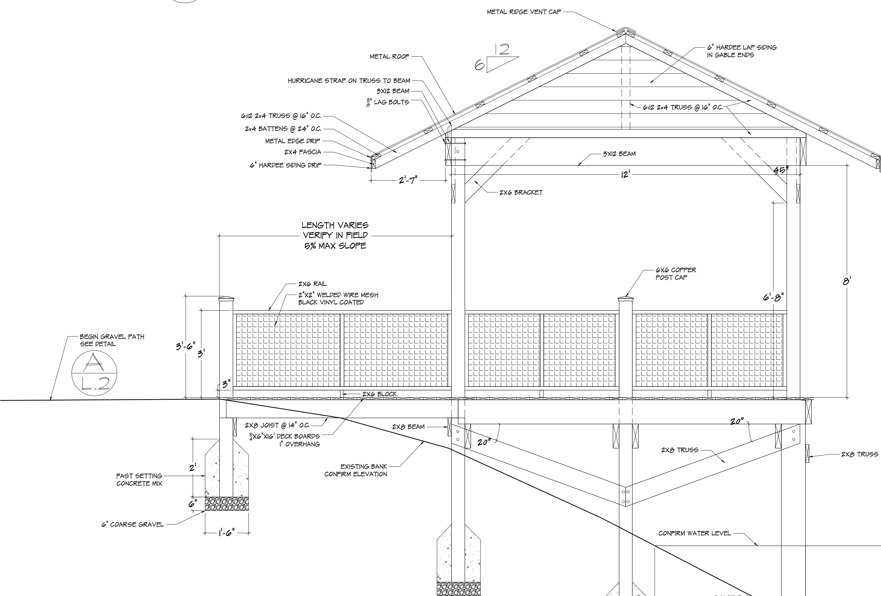
SIDE ELEVATION
