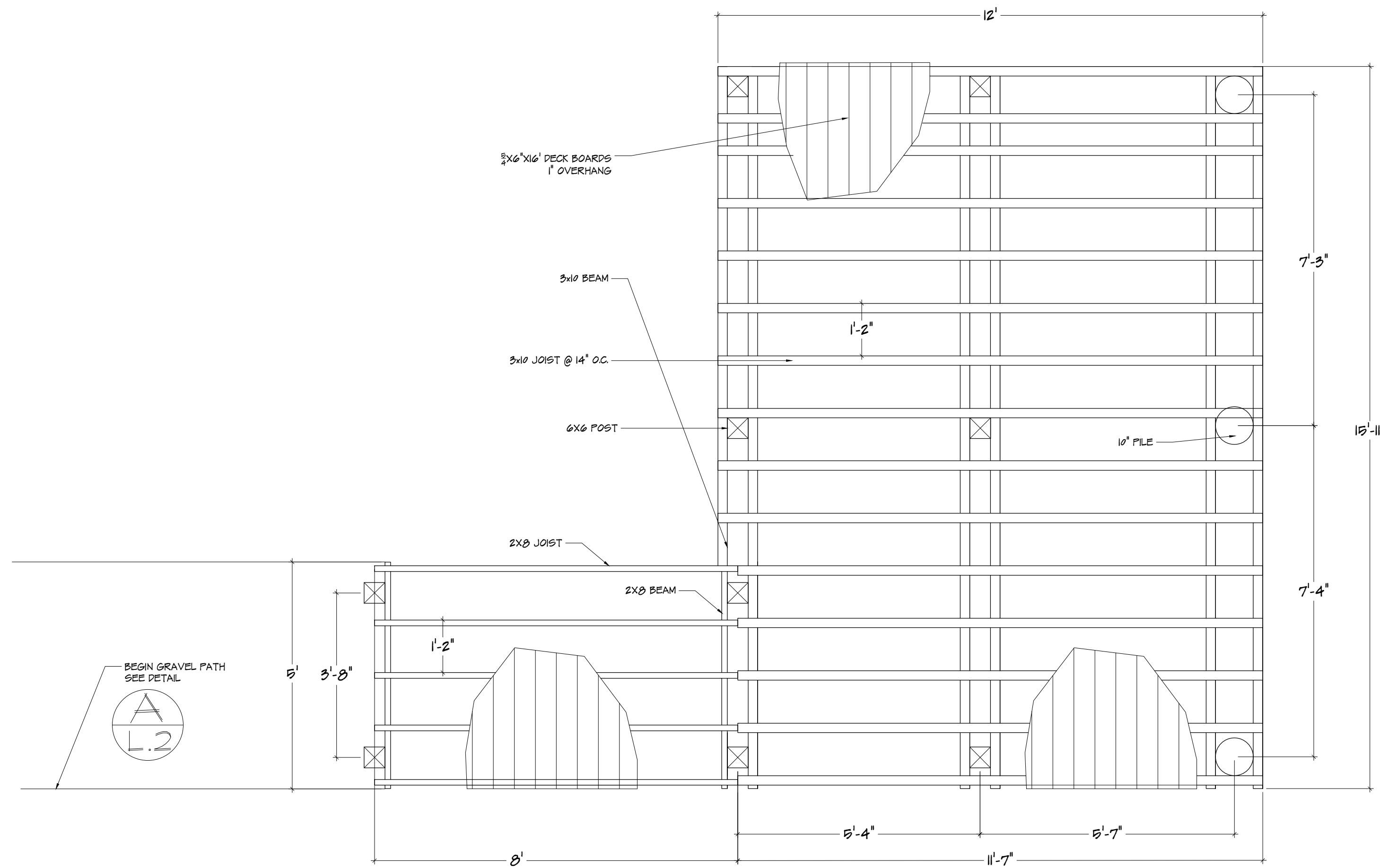
PLAN VIEW
